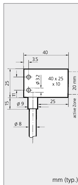
Winkel-Taster Angular scanner
